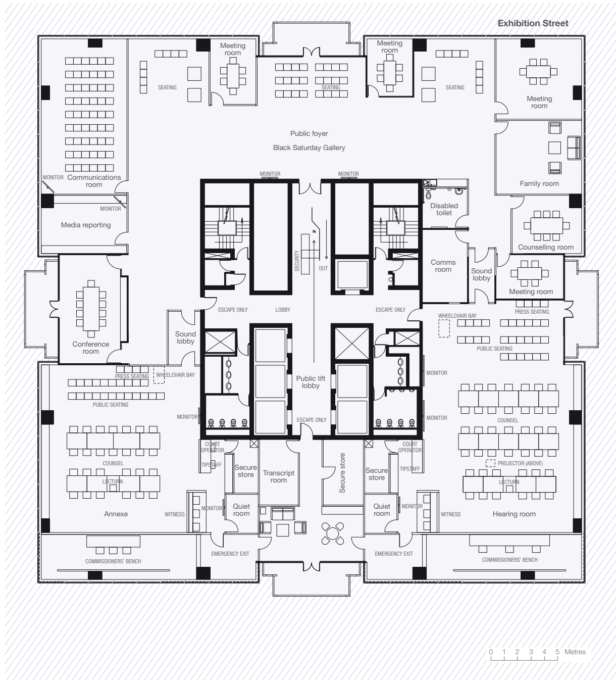
Figure F.1 Level 11 floor plan, Commission hearing rooms
